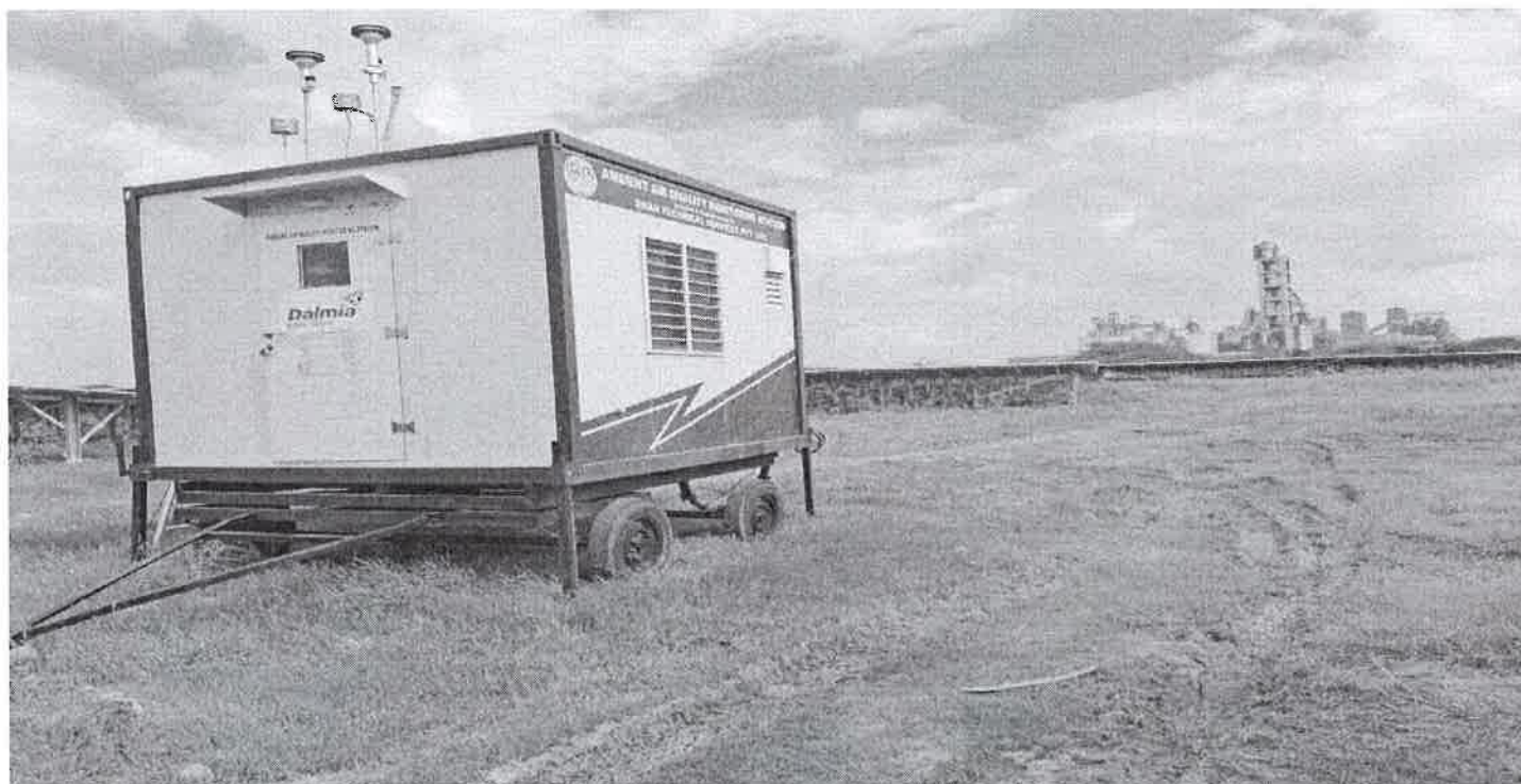
3 rd Movable CAAQMS
