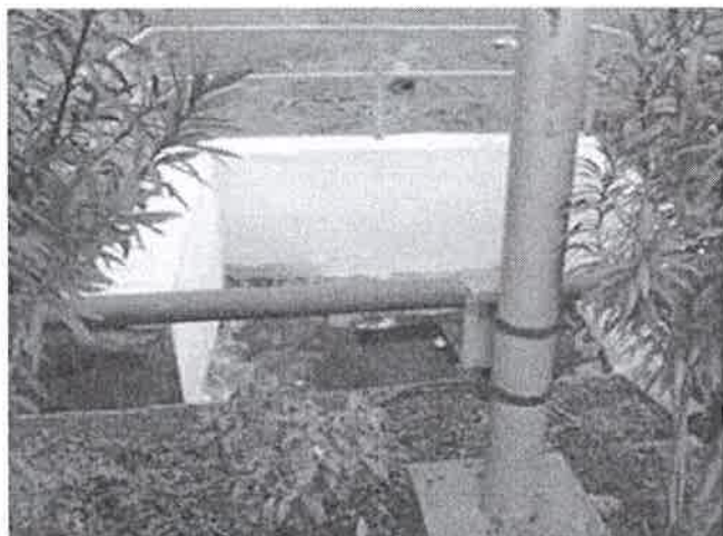
Drain Water Harvesting Pit
